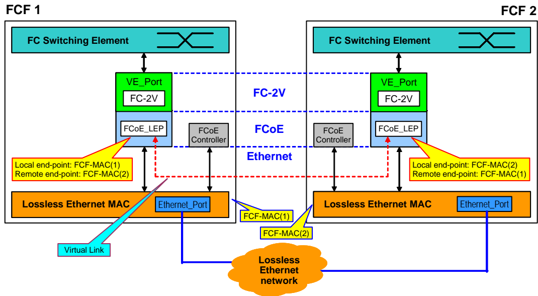
Figure 7 – VE_Port to VE_Port Virtual Links
