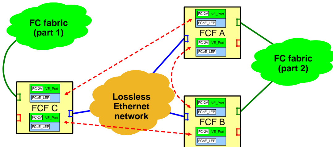
Figure 3 – FCoE VE_Port to VE_Port Network Configuration
