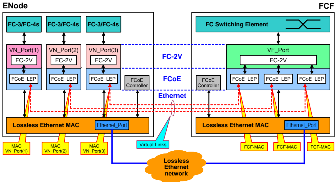
Figure 6 – VN_Port to VF_Port Virtual Links
