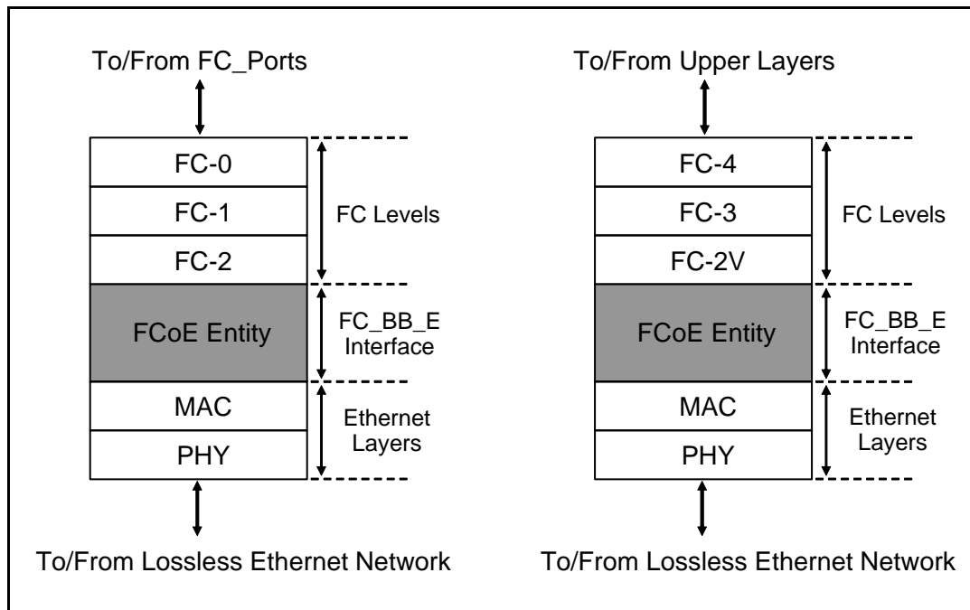
Figure 1 – FC-BB_E protocol levels and layers
