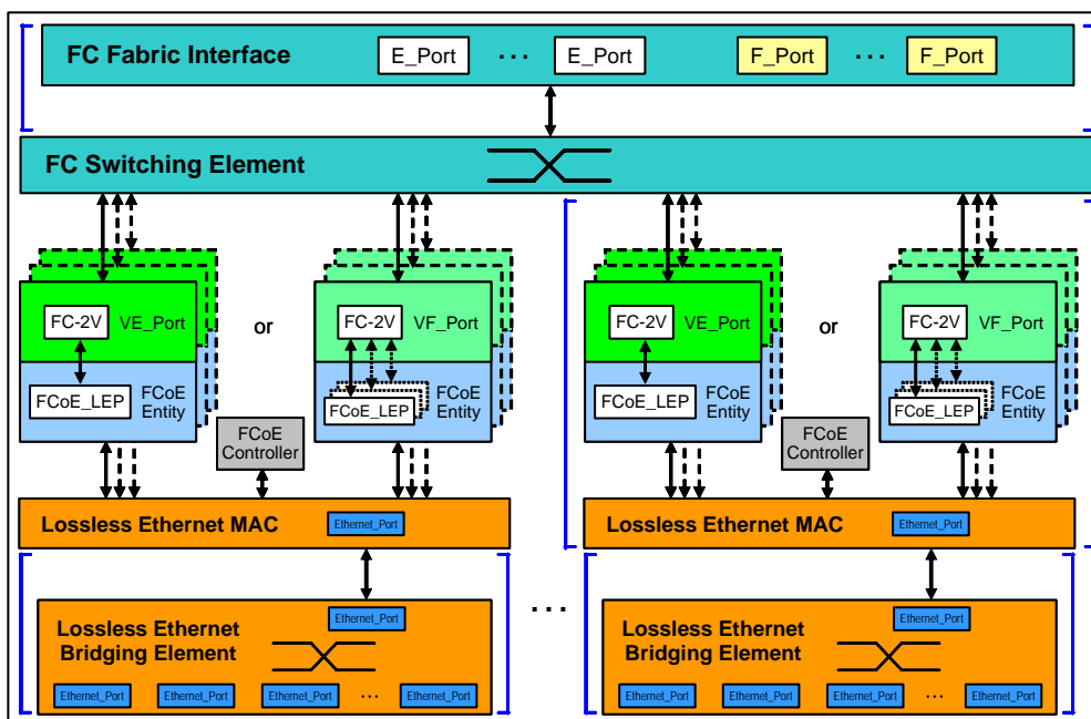
Figure 5 – FC_BB_E VE_Port/VF_Port functional model
