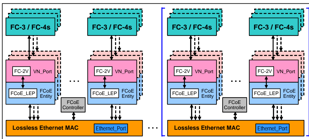
Figure 4 – FC_BB_E_VN_Port/ENode functional model
