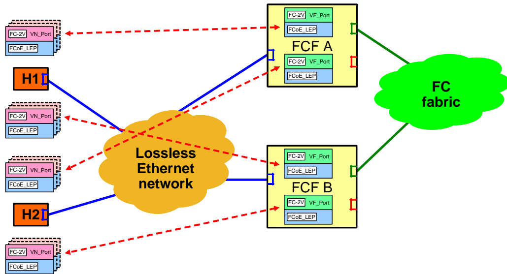
Figure 2 – FCoE VN_Port to VF_Port Network Configuration
